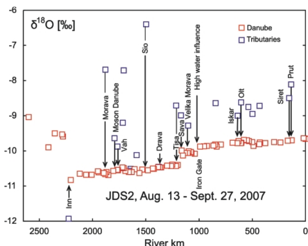
FIGURE 3: Longitudinal \delta^{18}\text{O} profile of the Danube (rkm 2600, Ulm – rkm 0, Black Sea) and \delta^{18}\text{O} values of tributaries at confluence (Aug. 13 – Sept. 27, 2007).
